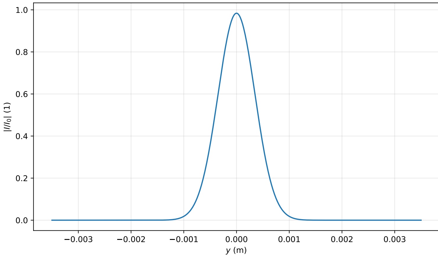
Intensity profile I(x=0, y, z=0.318)/I_0 , \text{Pin}=0.1\text{Pcr} , artificial time
